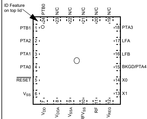
Pin connections
