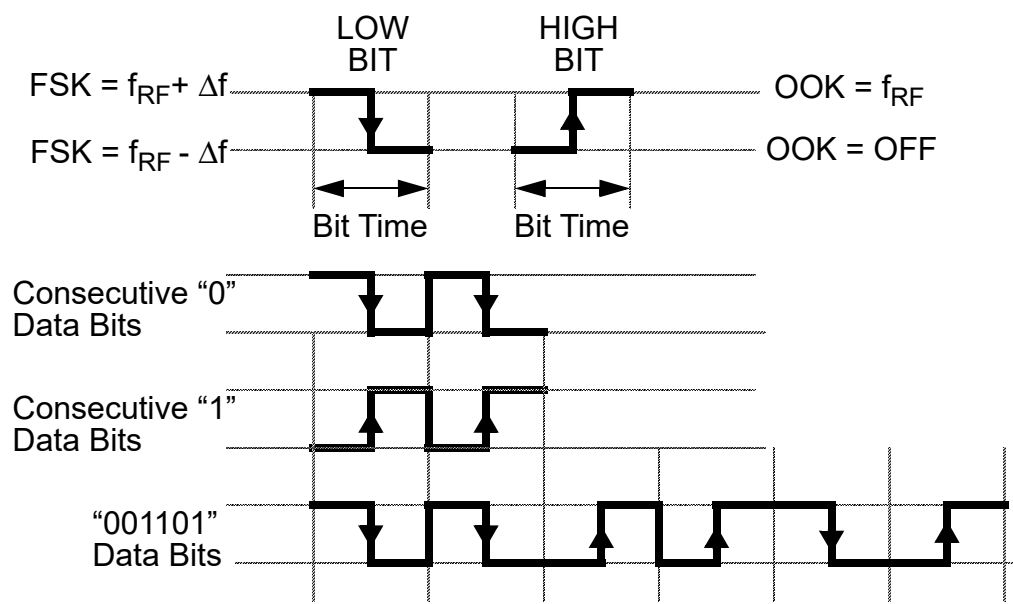
Figure 95. Manchester Data Bit Encoding (POL = 1)
