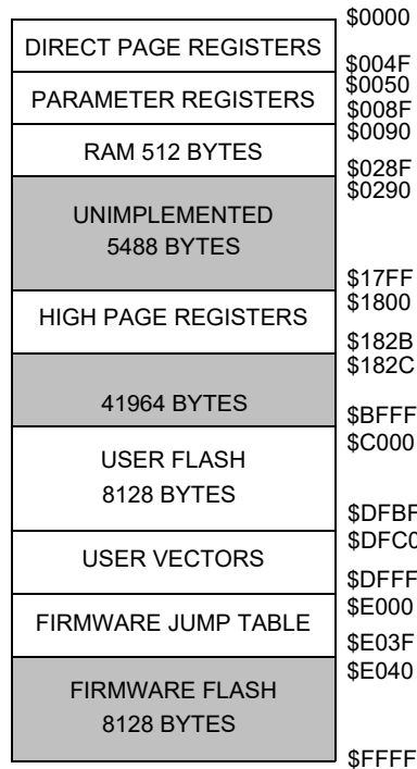
Figure 8. FXTH870x6 MCU Memory Map
