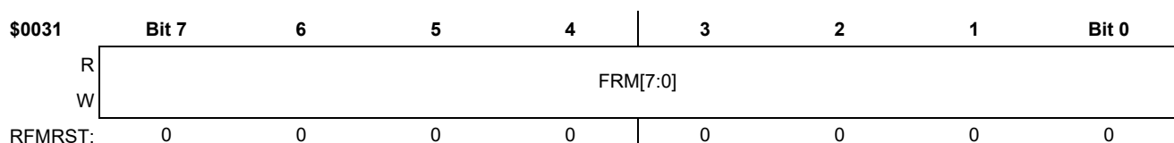
Figure 99. RFM Control Register 1 (RFCR1)
