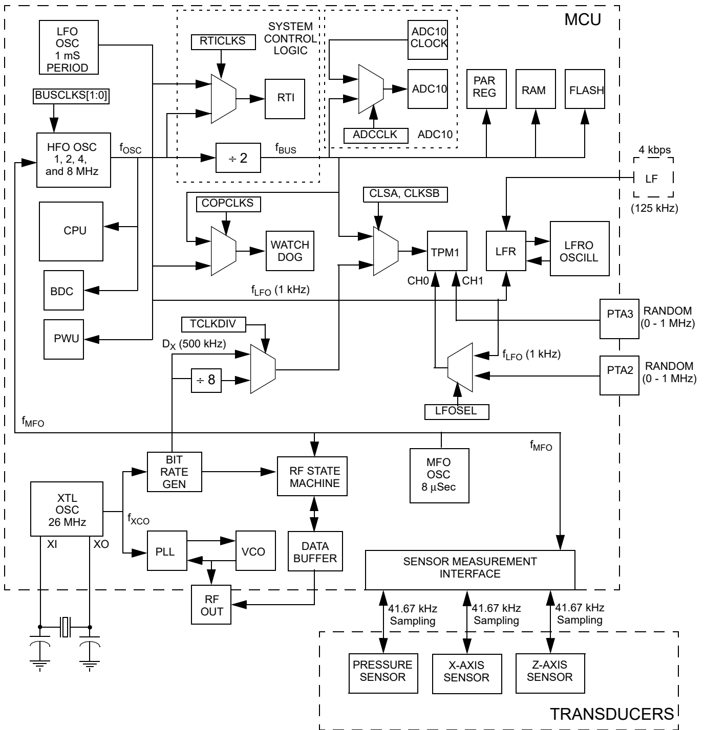
Figure 2. Clock Distribution
