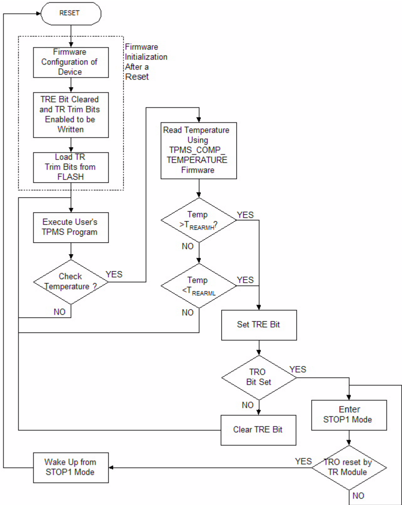
Figure 59. Flowchart for Using TR Module
