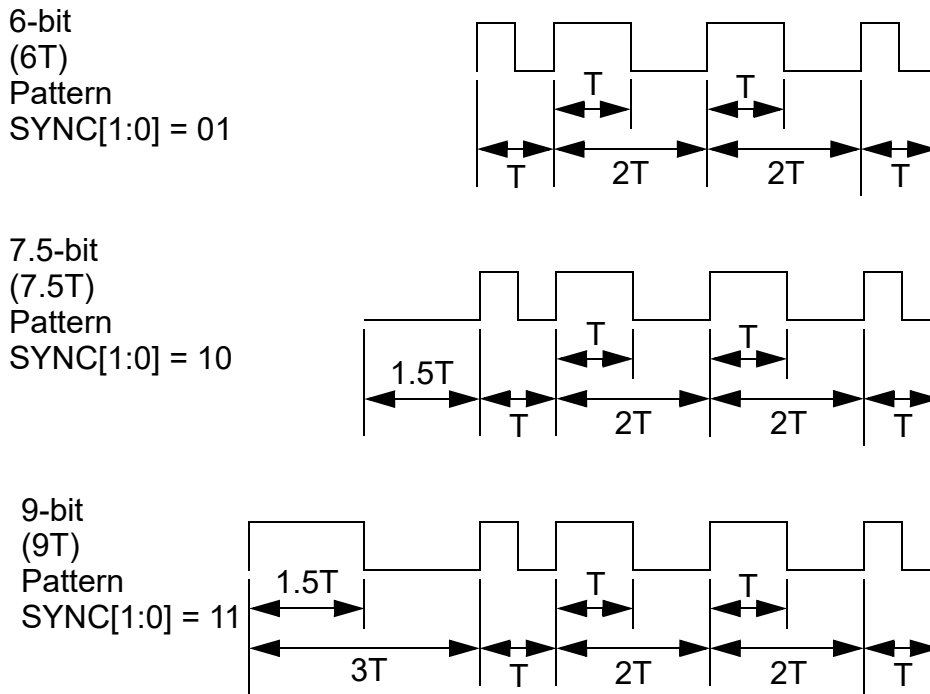
Figure 73. SYNC Patterns
