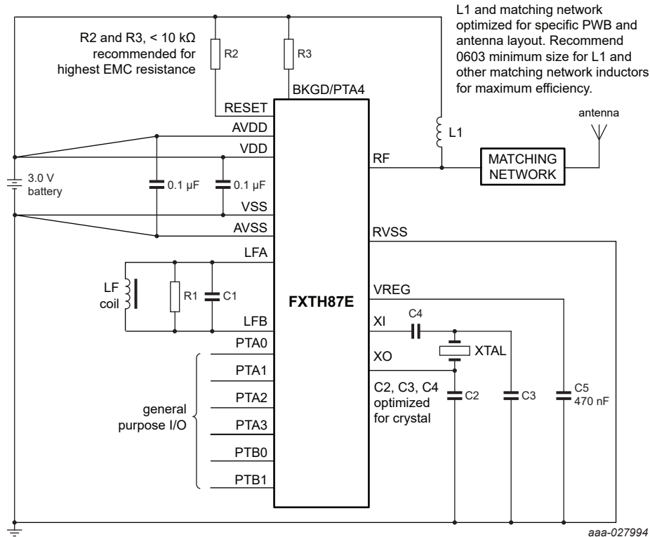
Figure 5. FXTH870x6 Example Application
