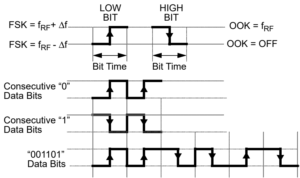
Figure 94. Manchester Data Bit Encoding (POL = 0)
